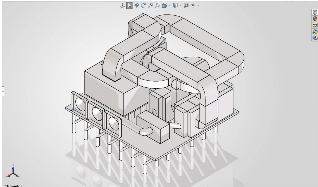
Figure 1. Concept CAD of the pier-mounted facility (SolidWorks): intake filter banks and mixing plenum, two Stage 1 rows of three 1.2 \times 1.2 \times 2.7 m plate-exchanger cores with their plenums, two air-to-seawater coils with Bay-water pipes through the deck, and the sealed server room with its return and supply ducting. One cooling path per row.
