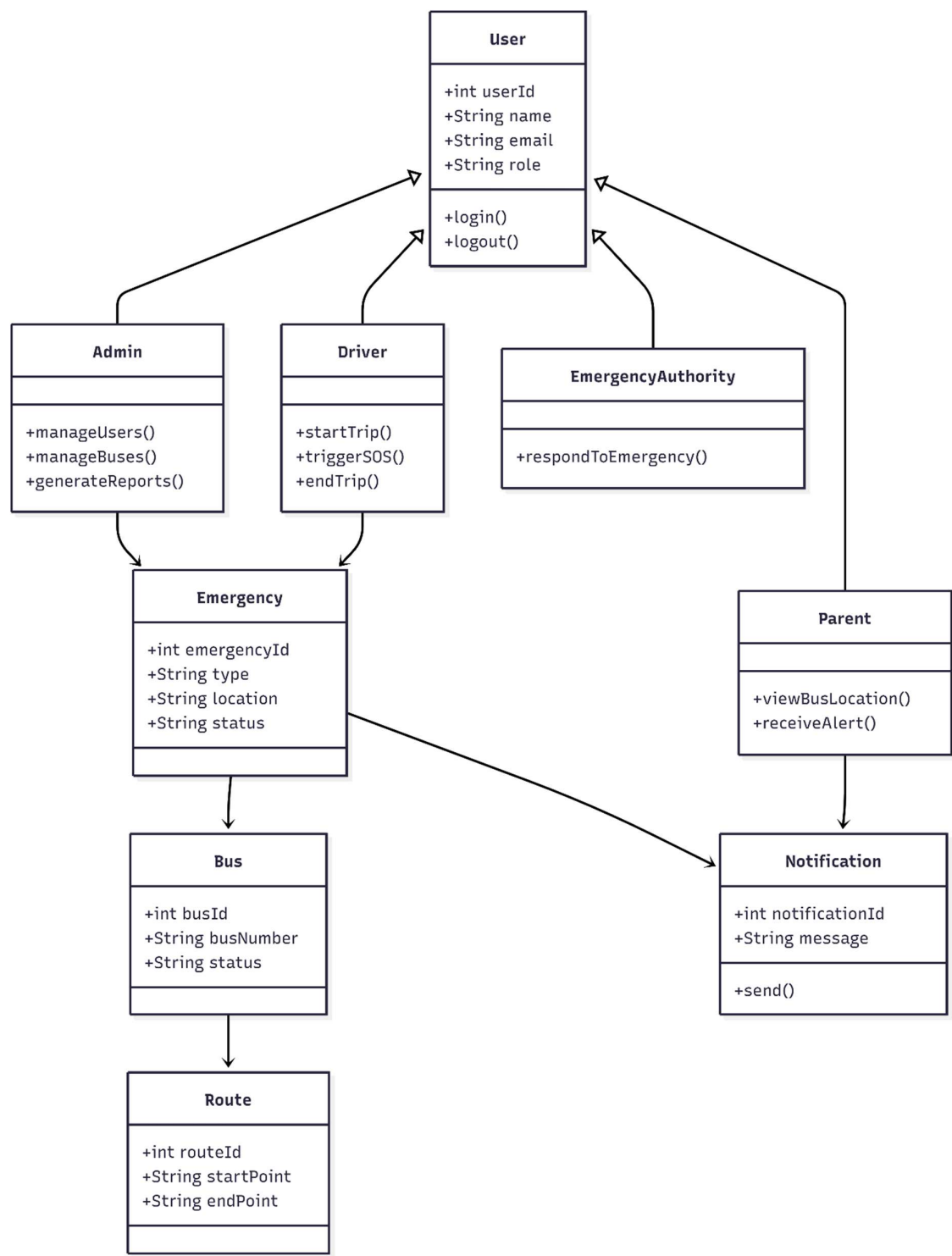
Class diagram
