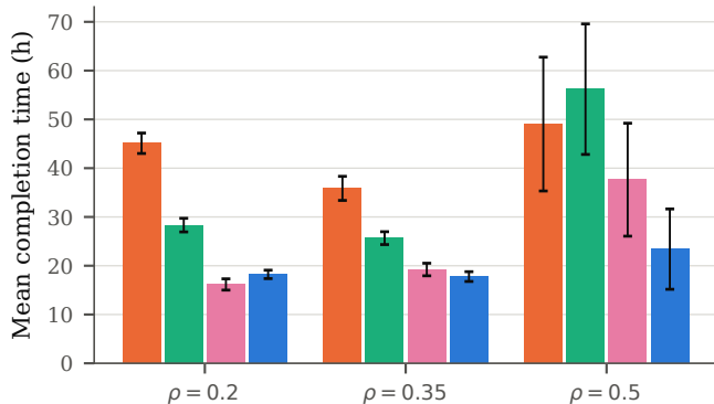
(b) Completion time of 4-GPU gang jobs
