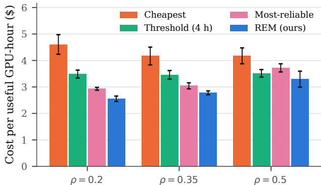
(a) Cost of 4-GPU gang jobs
