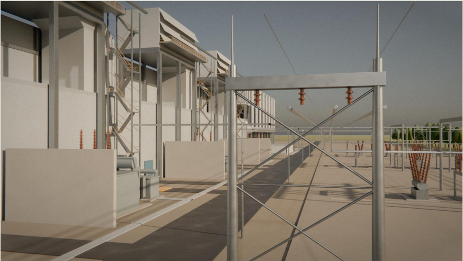
P2 — TRANSFORMER BAYS FROM THE ACCESS ROAD
