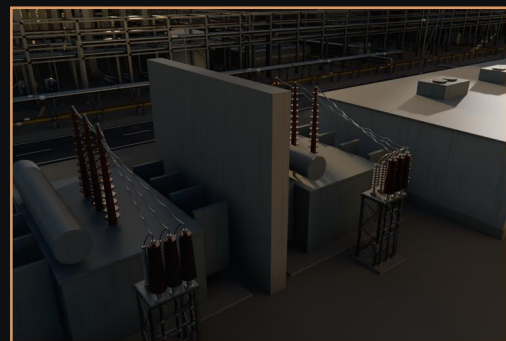
CCS transformers T-1 / T-2: 230 kV terminations and the tray riser
