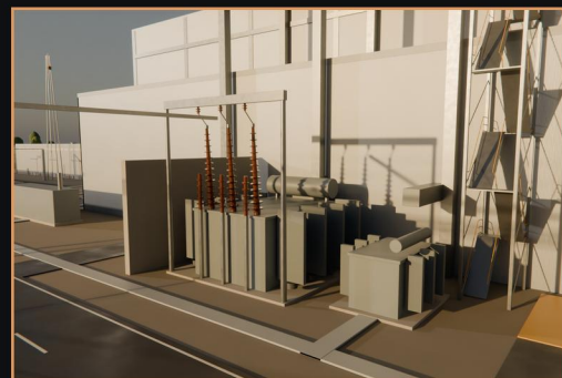
Generator step-up transformers facing the switchyard
