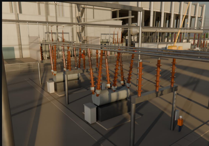
Bay D2: breakers, disconnects, trench to the relay house
