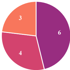
Hardware (n = 13)
