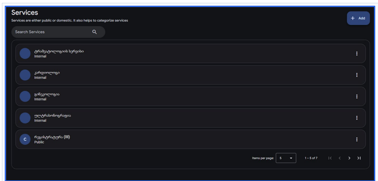
Fig. 6 — Service list
