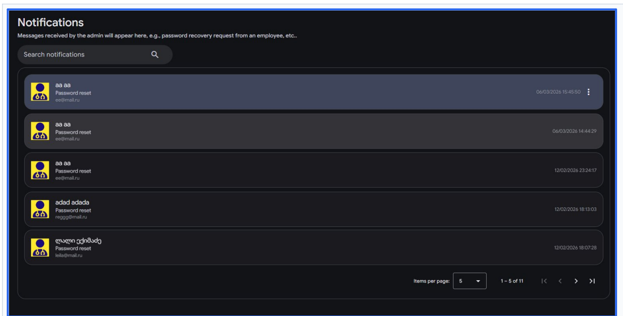
Fig. 15 — Notifications list
