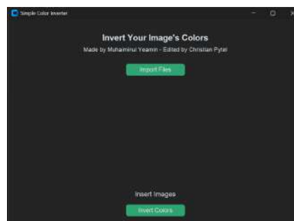
Figure 15: Inverting image colors for hologram generation.
