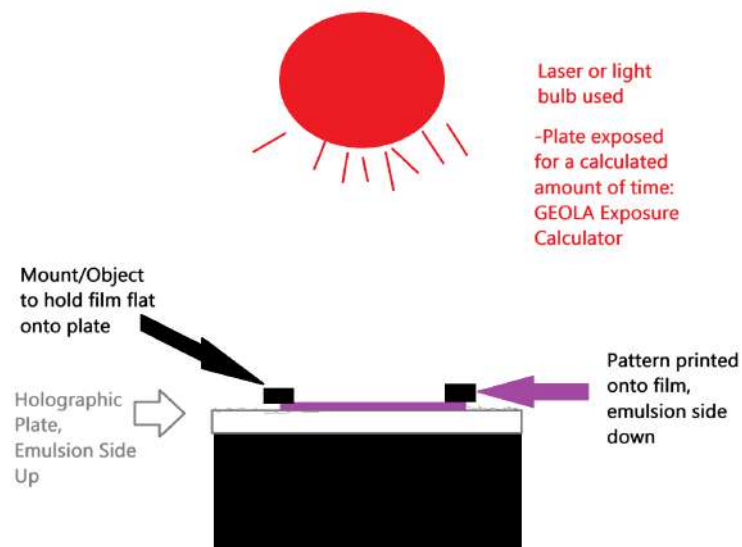
Figure 40: Exposing Holographic Plates
