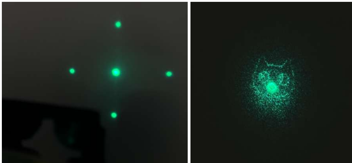
Figure 39: The beam after the grating and focused cat image.
