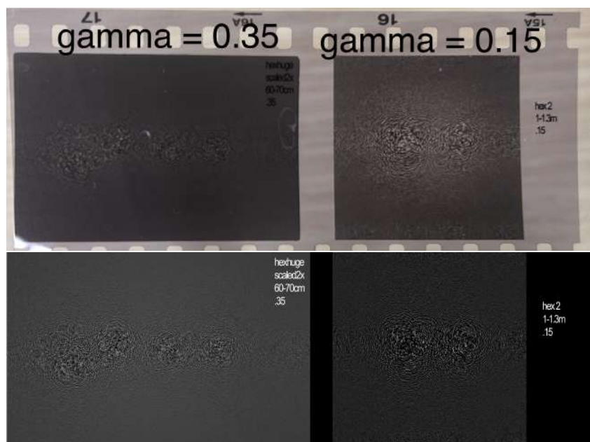
Figure 17: Using Gamma Correction on Film, with Original Images.
