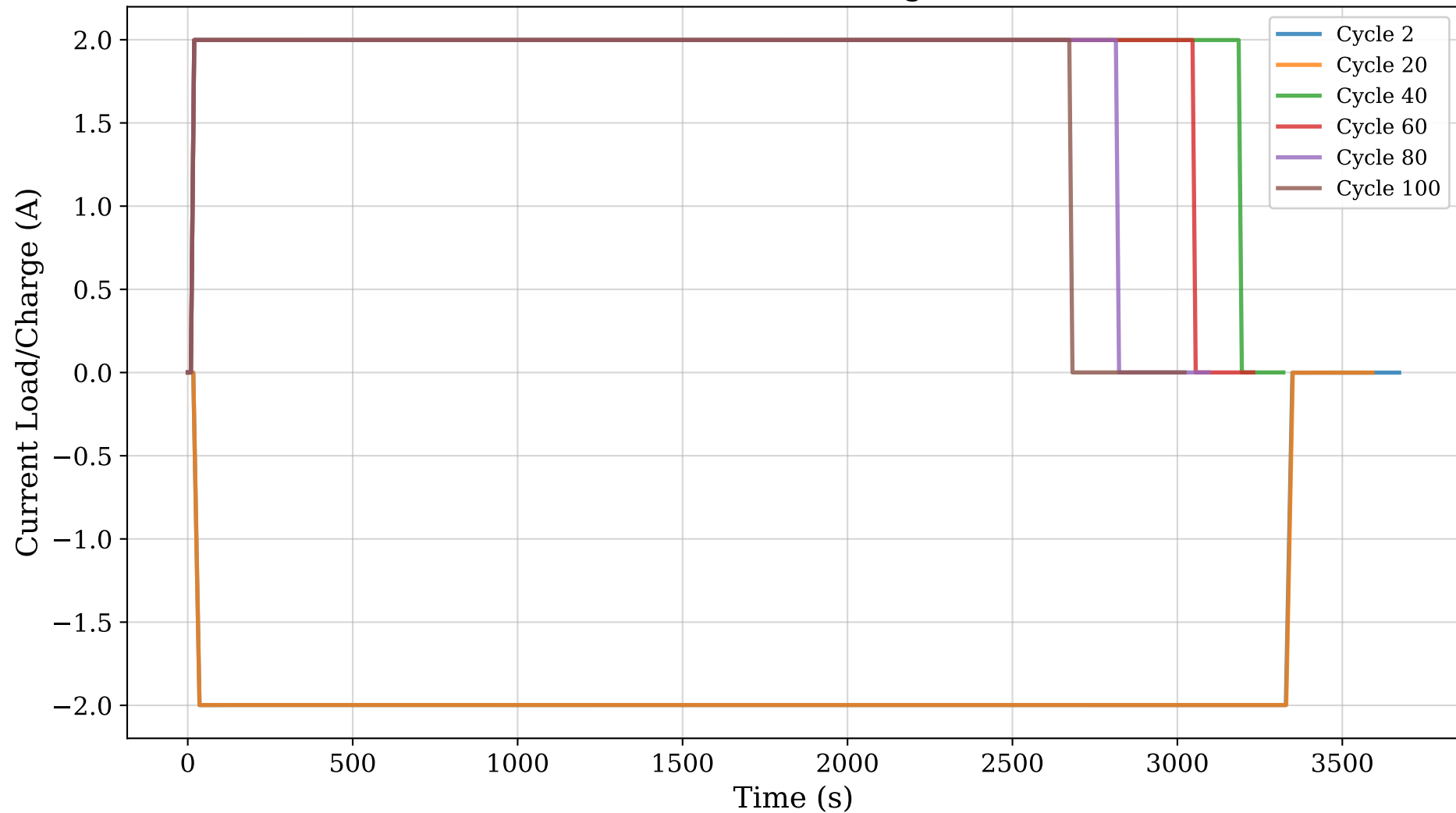
Current Load/Charge (A)
