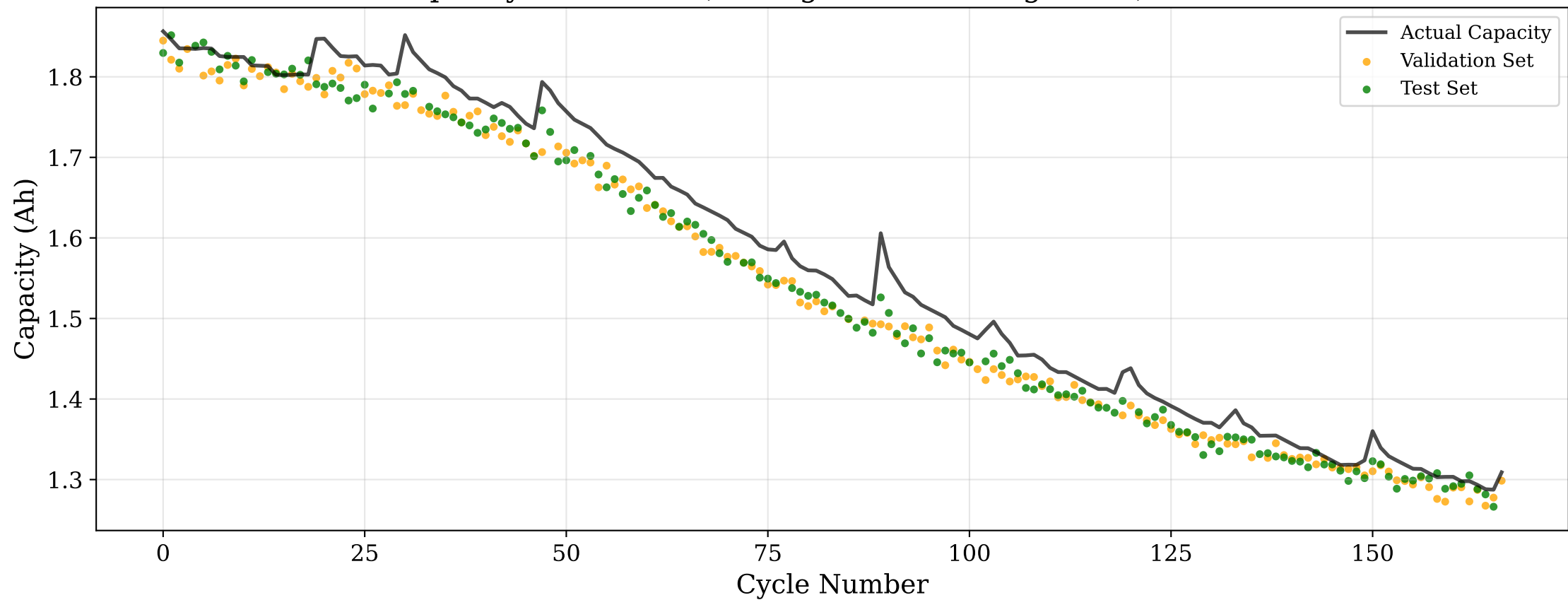
Capacity Prediction (Averaged over all segments) - B0005
