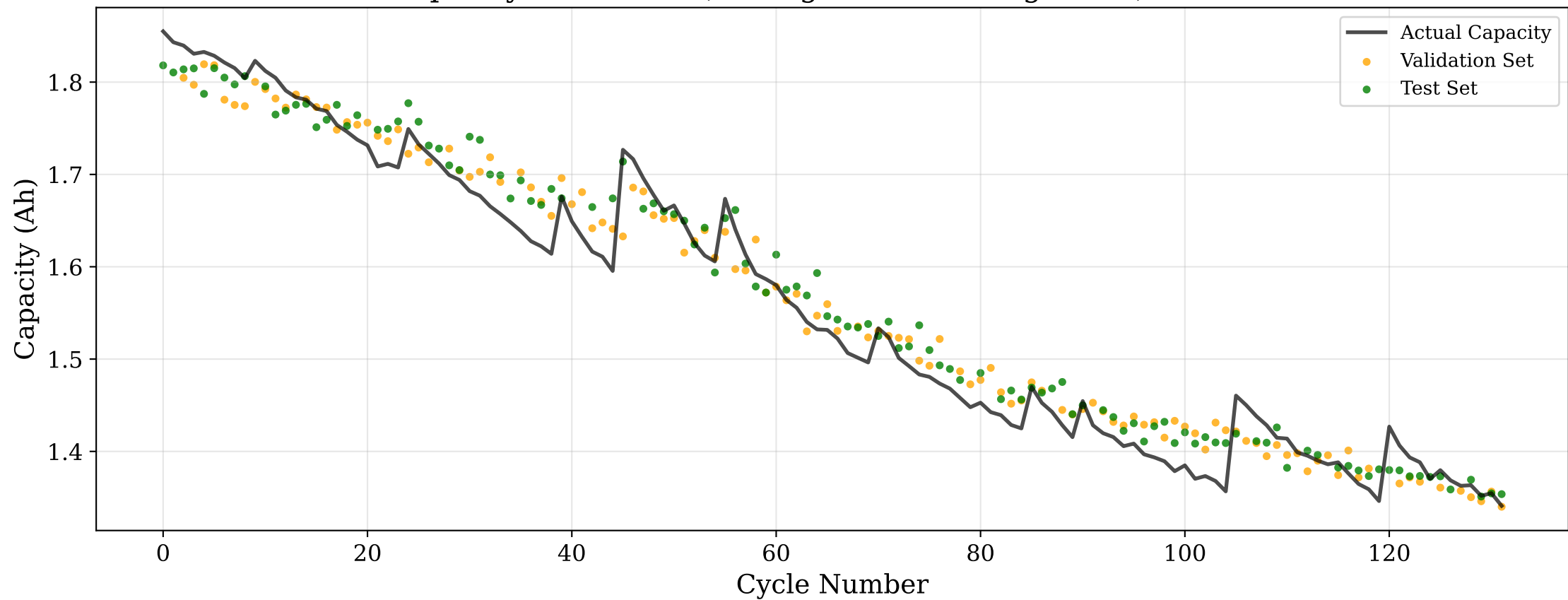
Capacity Prediction (Averaged over all segments) - B0018
