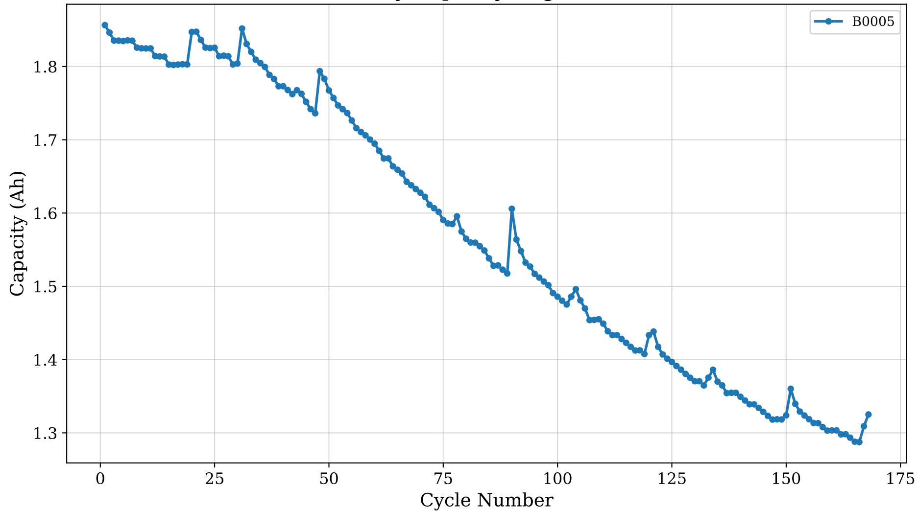
Battery Capacity Degradation
