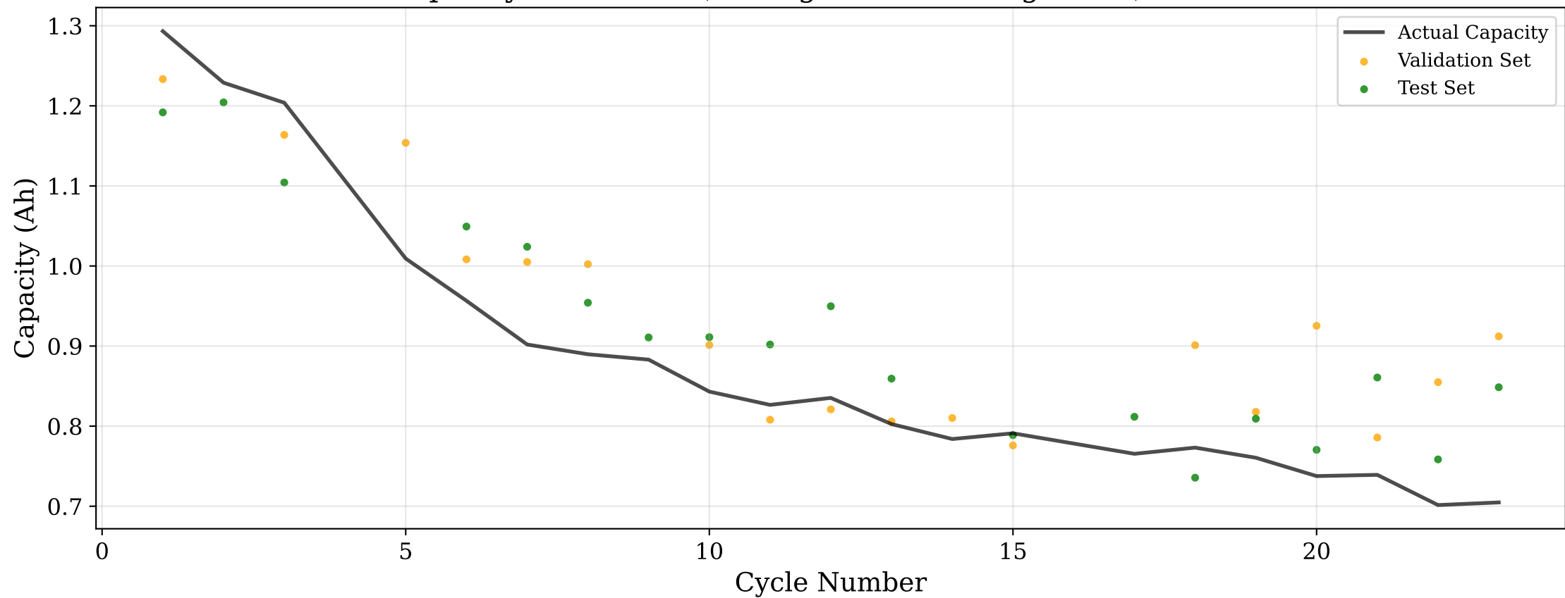
Capacity Prediction (Averaged over all segments) - B0051
