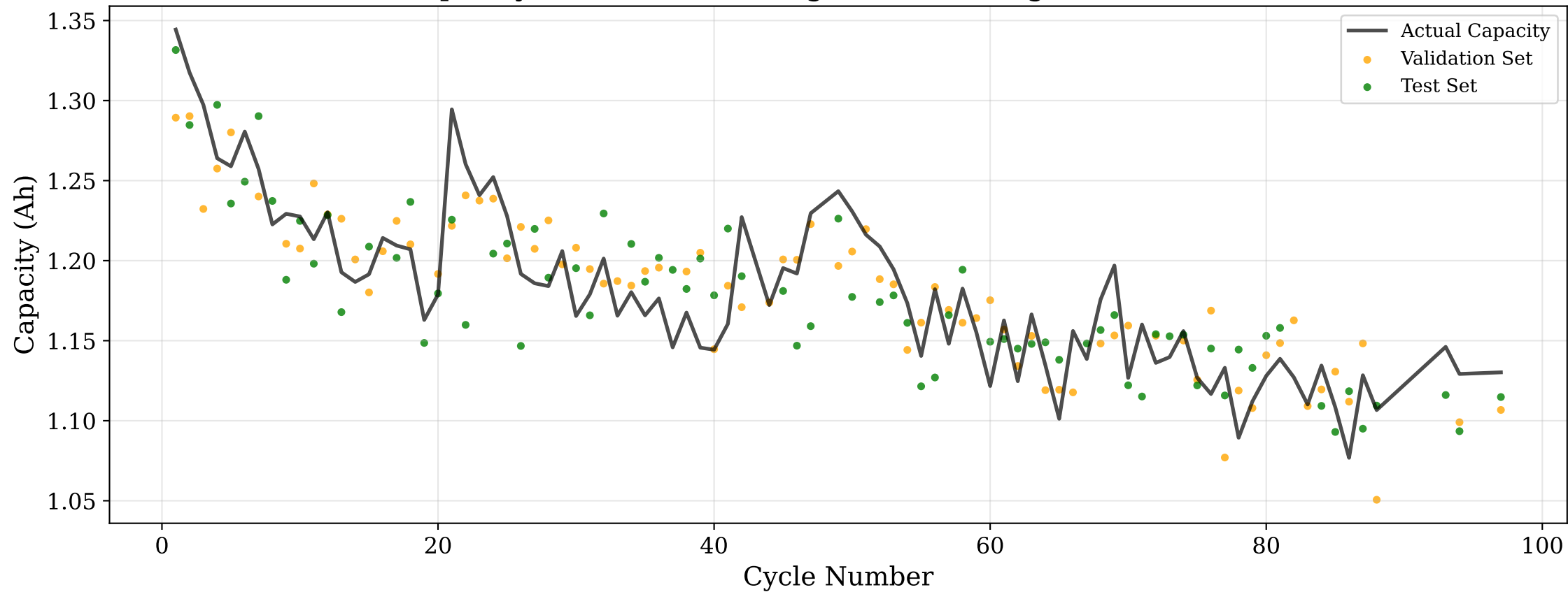
Capacity Prediction (Averaged over all segments) - B0056
