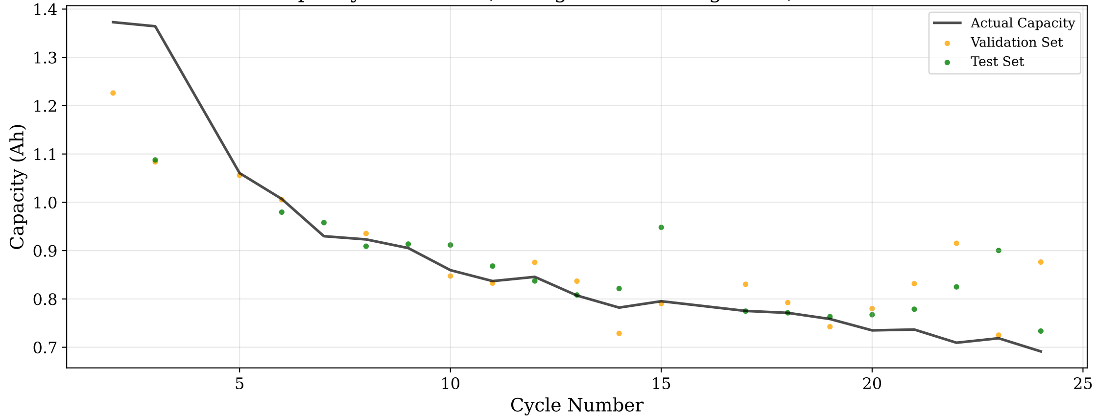
Capacity Prediction (Averaged over all segments) - B0049
