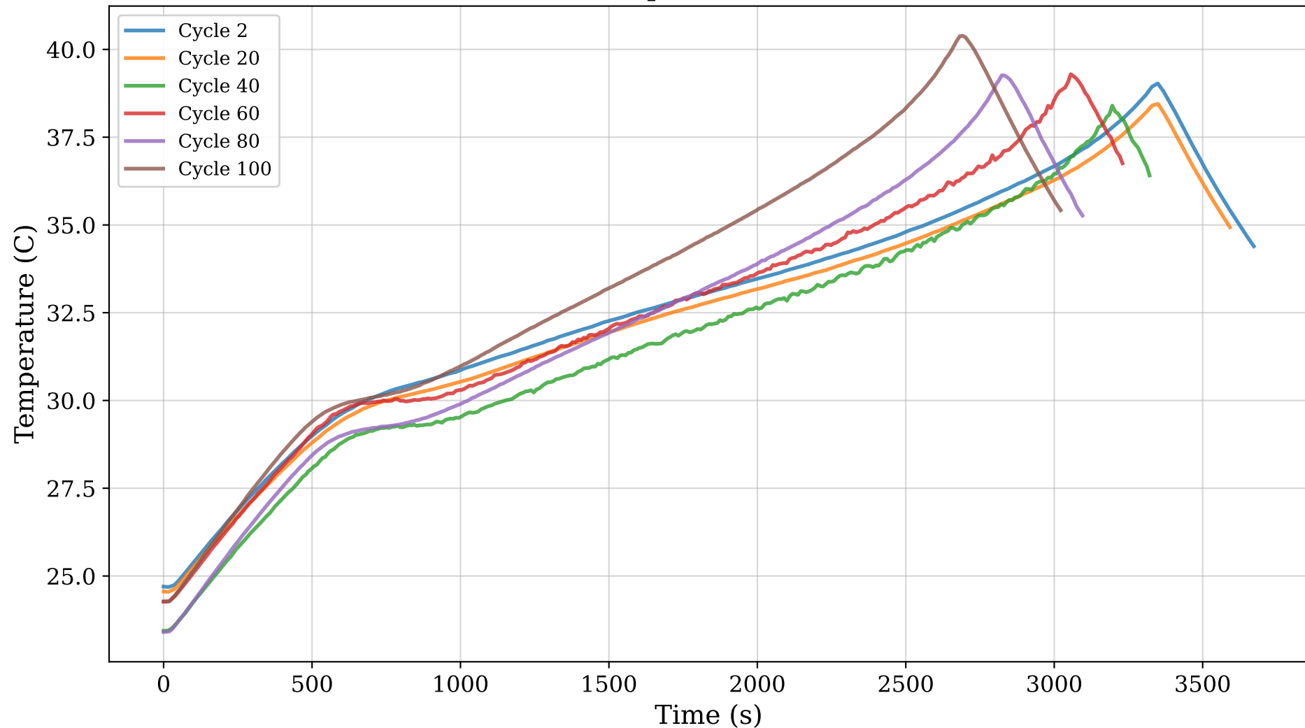
Temperature (C)
