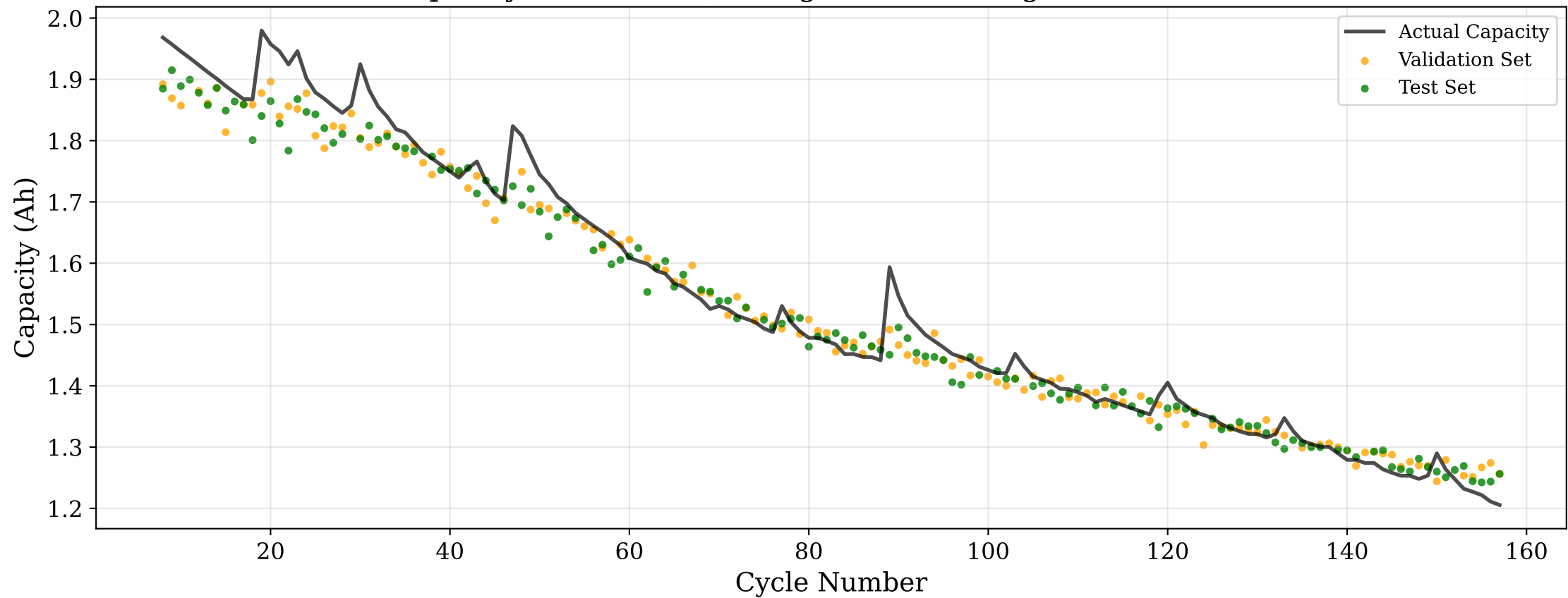
Capacity Prediction (Averaged over all segments) - B0006
