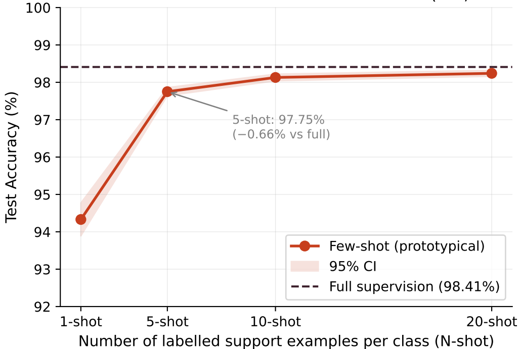
Few-Shot Generalisation — Groundnut Water Stress (HSI, 282 bands)
