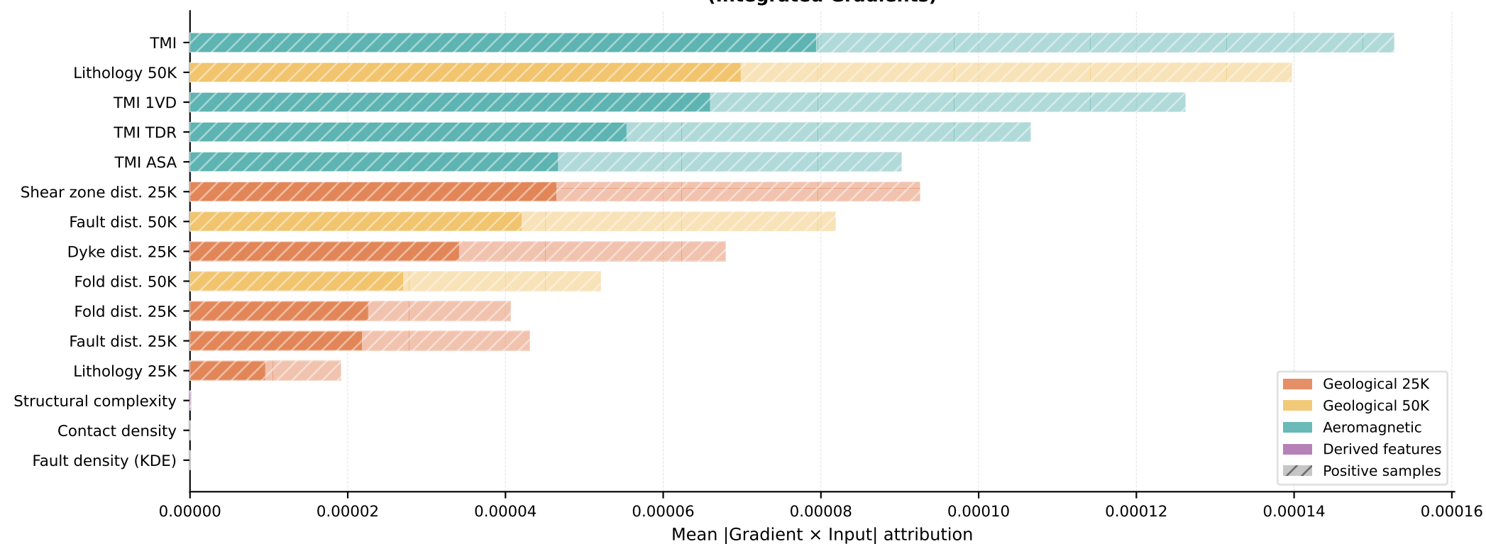
Figure 7 — Explainability Analysis: Channel Feature Importance Method: Integrated Gradients | n=300 samples (fold 0) | Depth: 0-500 m (a) Channel feature importance (Integrated Gradients)
