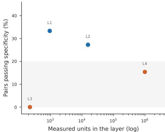
c More measurement does not rescue it
