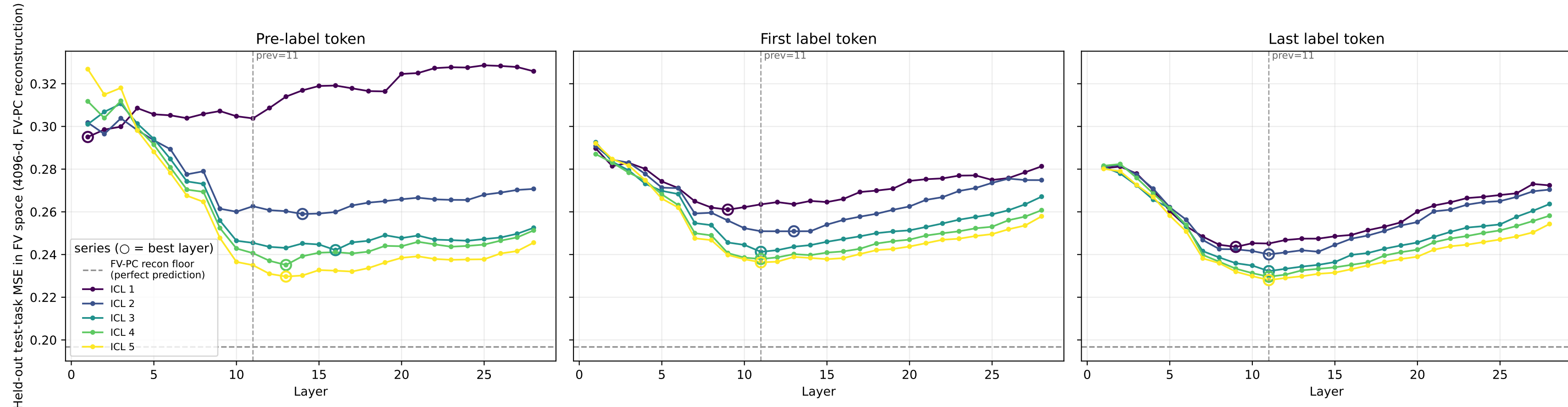
Layer sweep: OLS activation → function-vector regression, full-dim test MSE vs layer (activation PCs=16, FV PCs=16; MSE in 4096-d FV space; fit on train tasks → eval on held-out test tasks) (layers <1 omitted: embedding layer MSE is off-scale)
