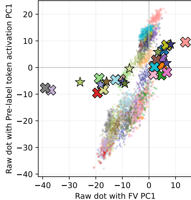
Pre-label token
