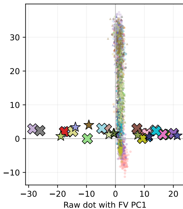
Pre-label token
