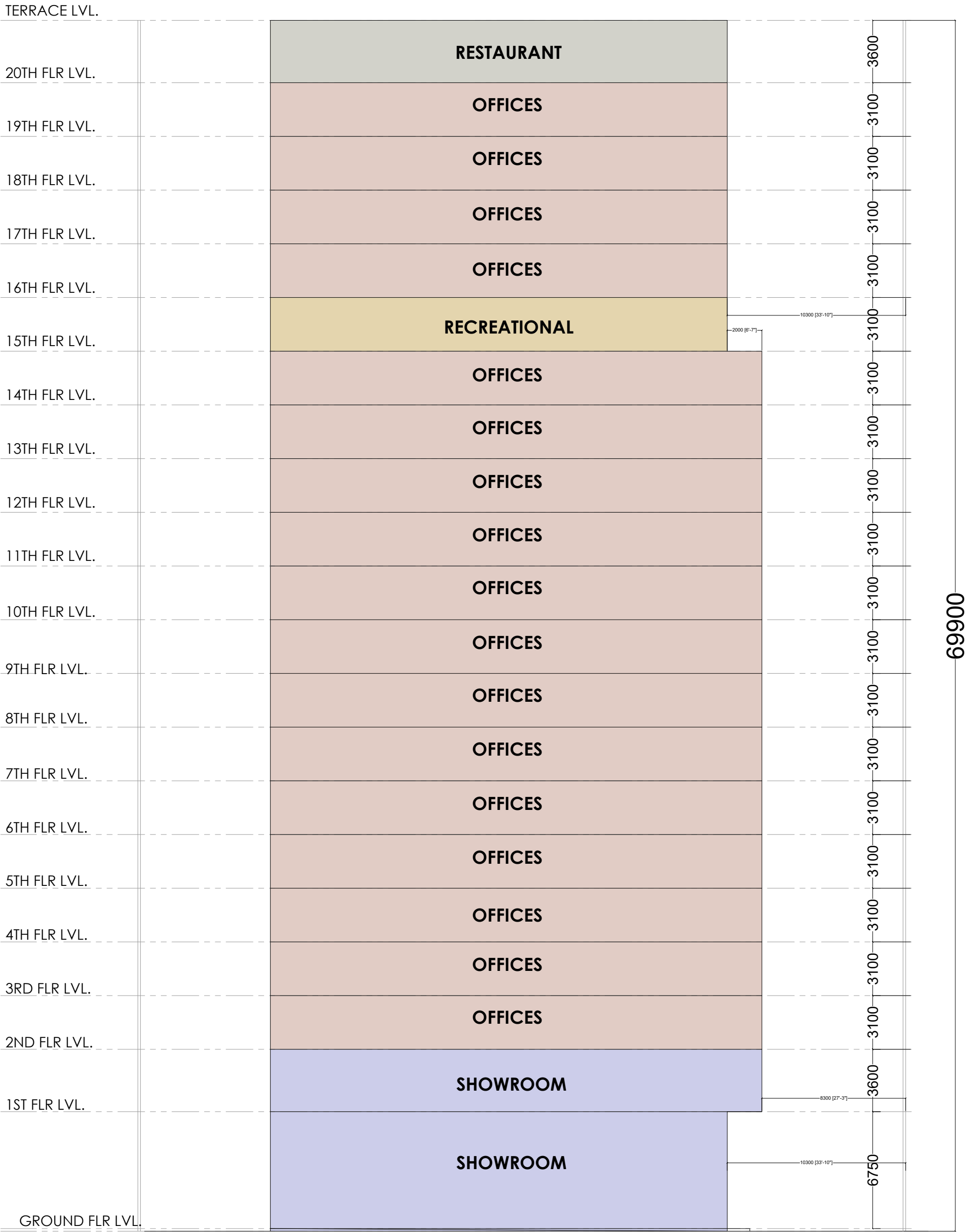
SCHEMATIC SECTION
