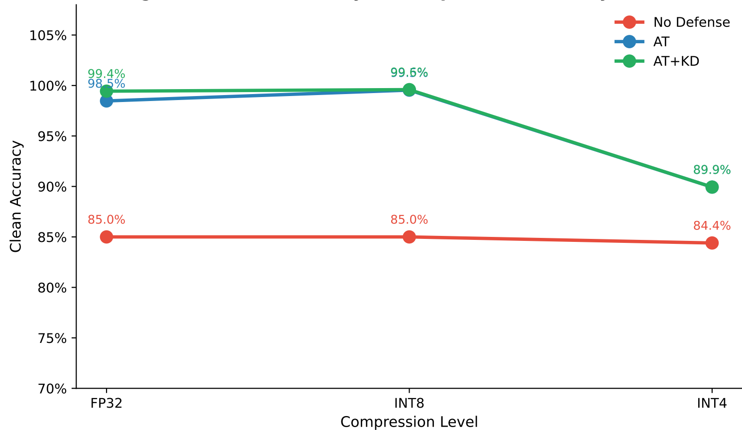
Figure 7: Clean Accuracy vs Compression Level by Defense
