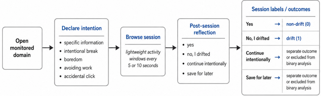
Fig. 2. DriftSense session-labeling flow. Prompted conditions ask users to declare an intention before a monitored-domain session and later report whether the visit matched that intention. The passive condition uses a retrospective post-session drift label.
