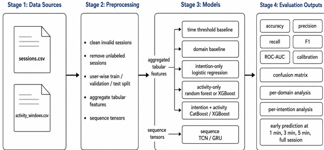
Fig. 3. Planned DriftSense modeling and evaluation pipeline. Exported session and activity-window data are cleaned, split, transformed into first-3-minute and full-session tabular features, evaluated across baselines and intention-aware models, and used to support model-assisted reflective check-ins.
