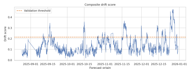
FIGURE 7. DFEH composite distribution-shift score timeline across the test holdout, with the fixed validation-calibrated 0.90-quantile threshold.
