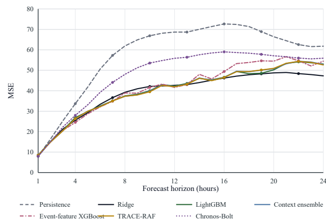
FIGURE 5. MSE by forecast lead time ( h = 1 to h = 24 ) across principal models on the test holdout.
