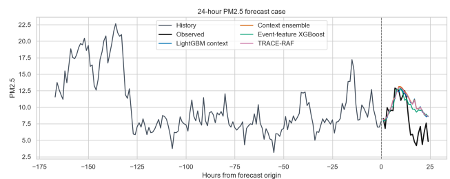
FIGURE 8. Representative test forecast origin under ordinary conditions: base ensemble, TRACE-RAF correction, and observed ground truth.
