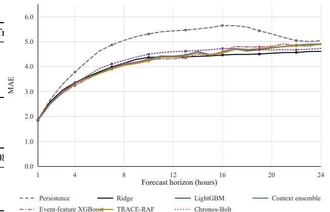
FIGURE 6. MAE by forecast lead time ( h = 1 to h = 24 ) across principal models on the test holdout.
