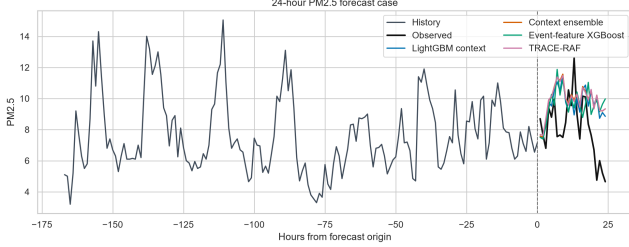
Fig. 9. Representative forecast whose target lies within the declared 72-hour event-context window. The event designation is retrospective because Storm Events files do not expose publication timestamps.
