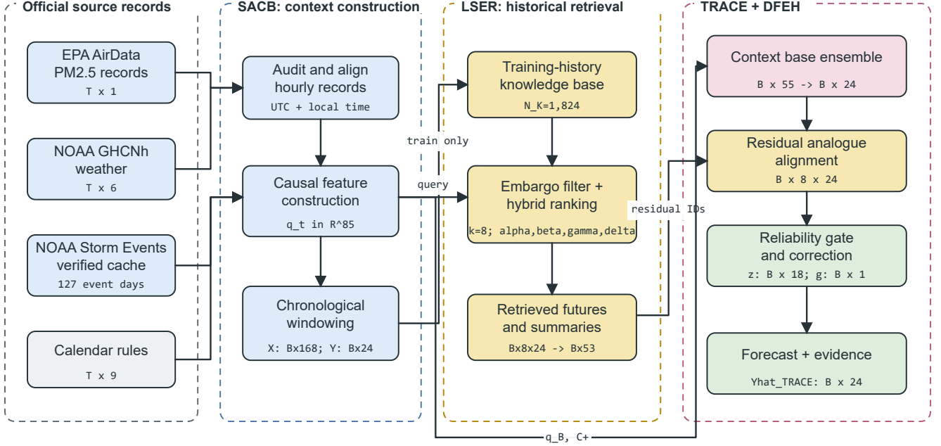
Fig. 1. Proposed TRACE-RAF pipeline. Official records pass through SACB, training-history candidates are filtered and ranked by LSER, out-of-fold residual analogues are scaled by the TRACE trust gate, and DFEH produces the 24-hour forecast with traceable evidence. Tensor annotations show the manifest-backed configuration.
