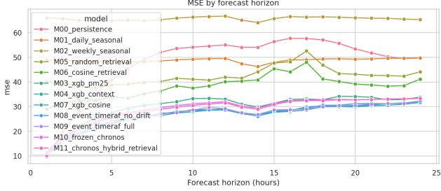
Fig. 6. MSE by forecast horizon on the Los Angeles County test set.
