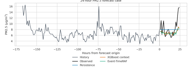
Fig. 9. Representative 24-hour forecast case from the test set.
