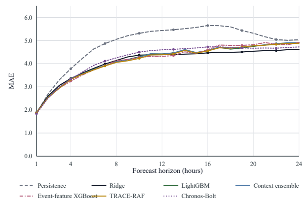
FIGURE 6. MAE by forecast horizon on the Los Angeles County test set.
