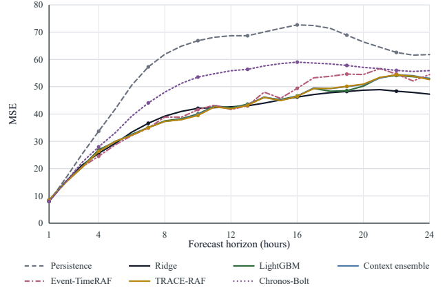
Fig. 5. MSE by forecast horizon on the Los Angeles County test set.
