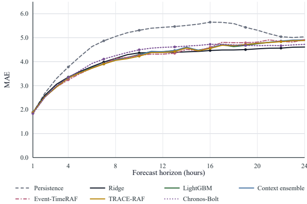
Fig. 6. MAE by forecast horizon on the Los Angeles County test set.
