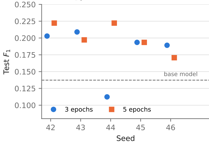
(b) Test F_1 per seed
