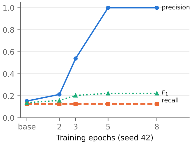
(a) Epoch sweep
