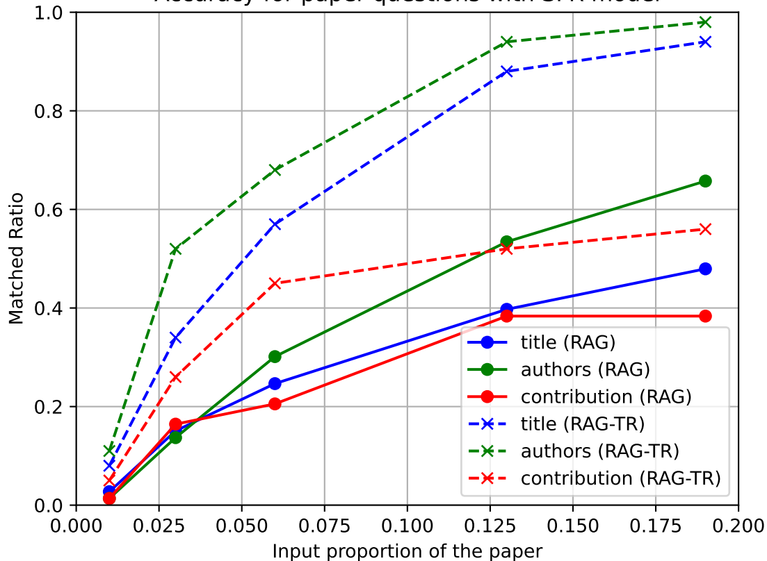
Accuracy for paper questions with SFR model
