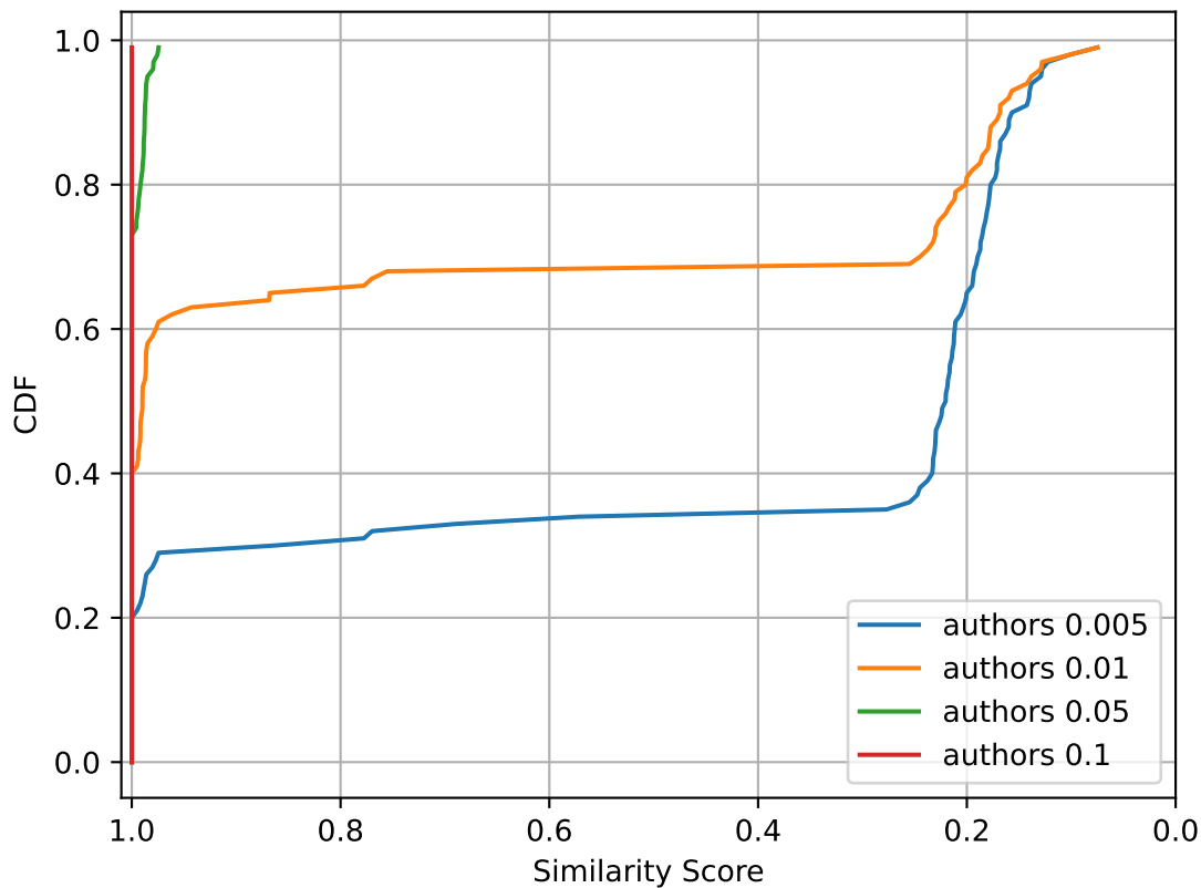
CDF for authors
