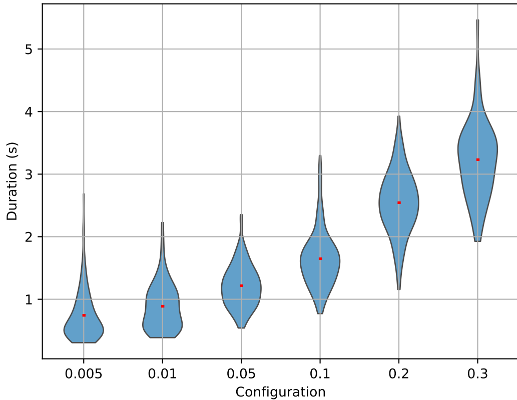
Violin Plot of Duration for authors
