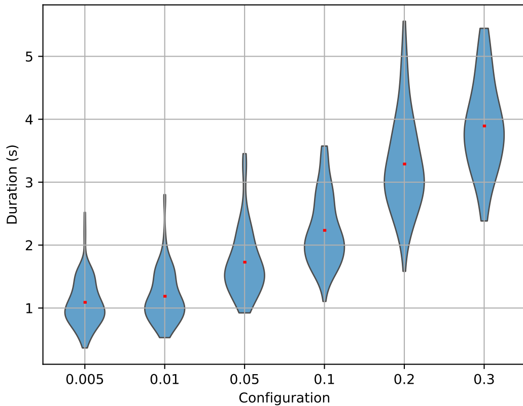
Violin Plot of Duration for contribution
