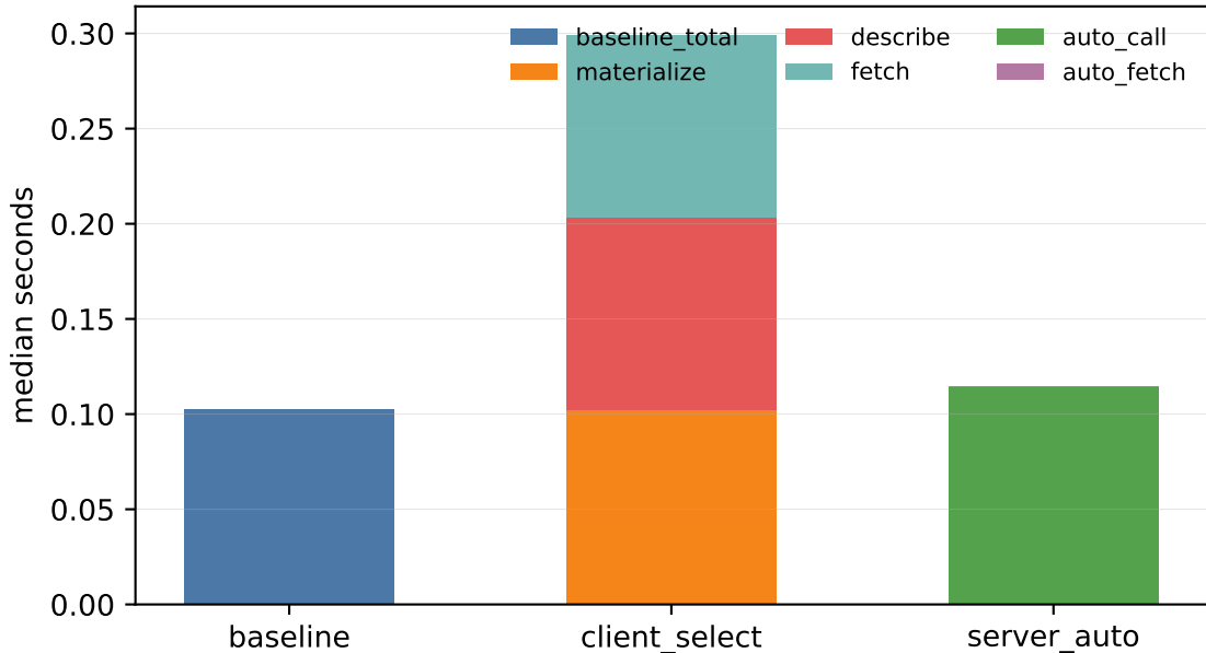
Median overhead breakdown (BIRD server-exec)
