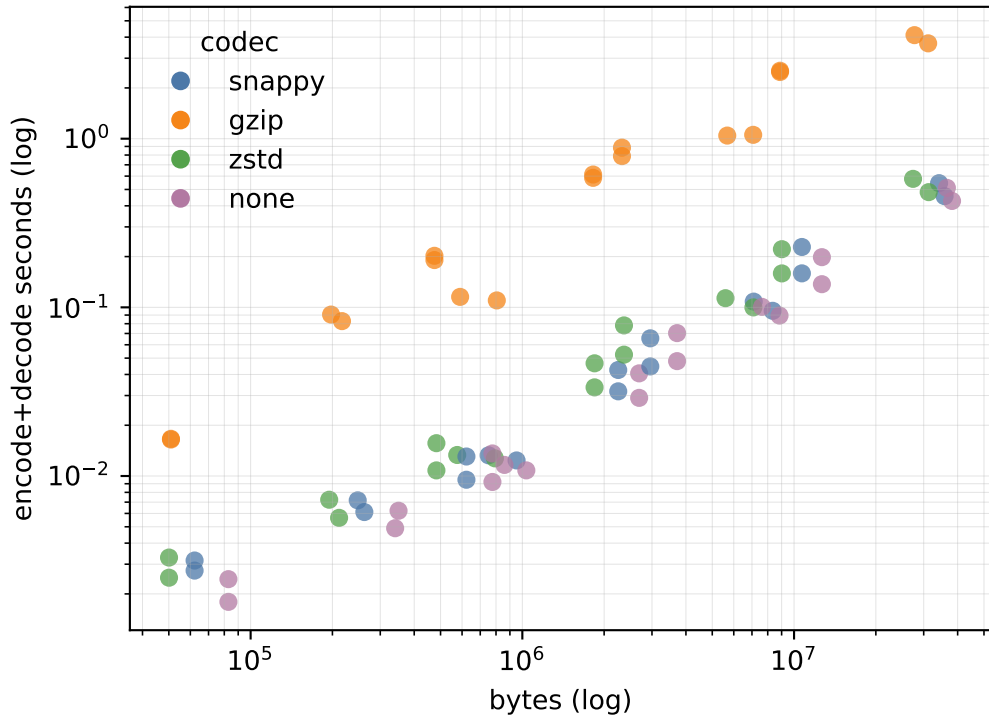
Codec trade-off: size vs (encode+decode)
