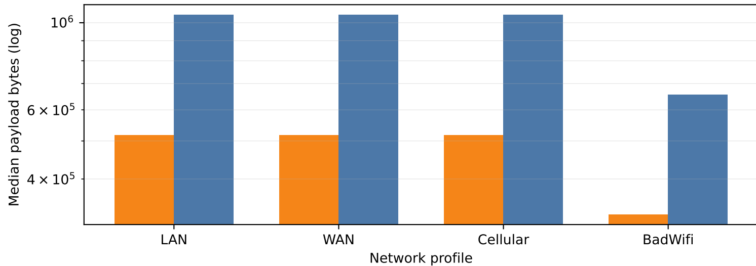
Structured vs unstructured: payload by network
