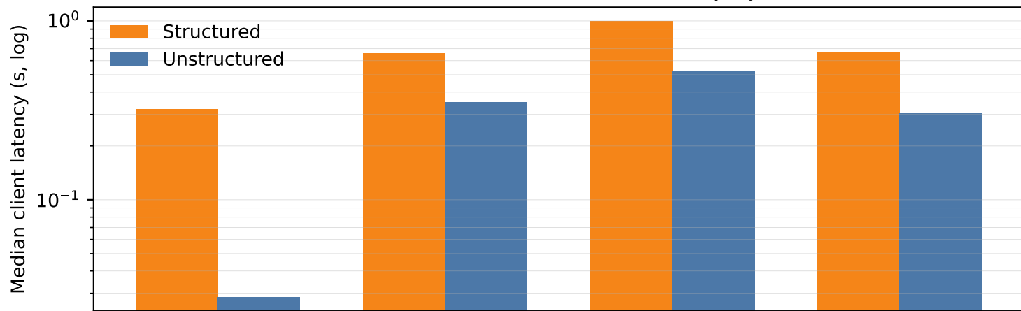
Structured vs unstructured: client latency by network
