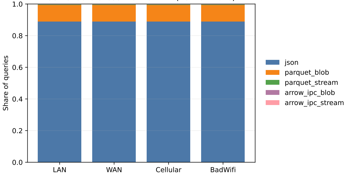
Server-auto chosen format mix (network runs)
