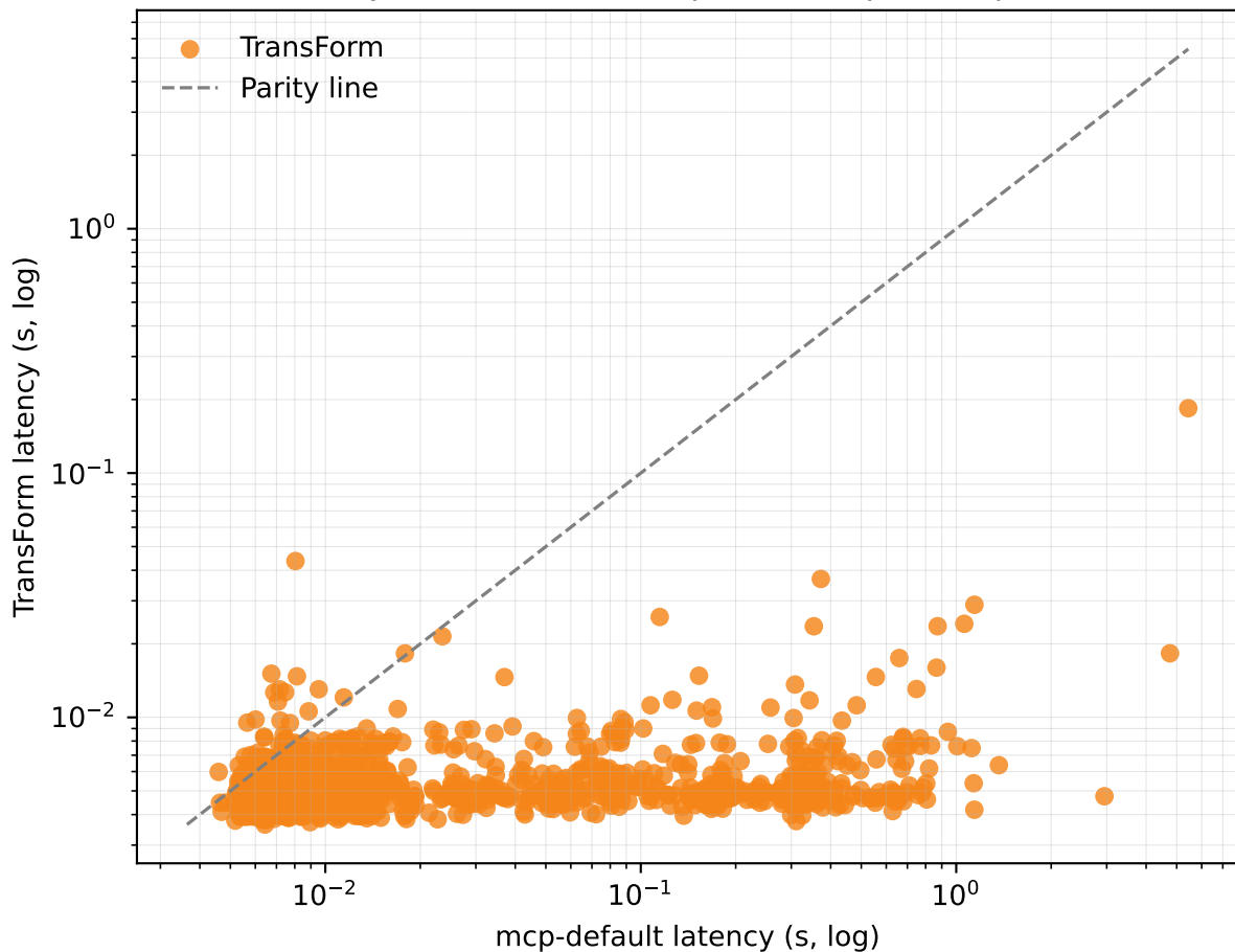
Latency: TransForm vs mcp-default (paired queries)
