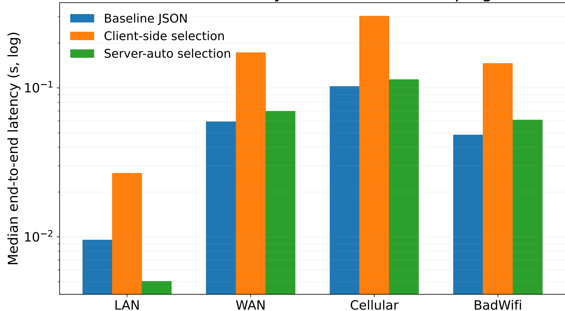
BIRD E2E latency under network shaping
