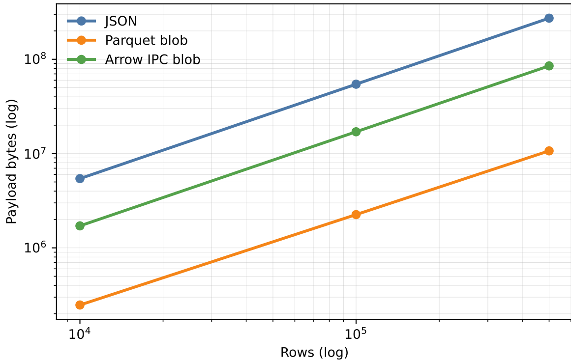
Payload size comparison (TPC-DS, 20 columns)
