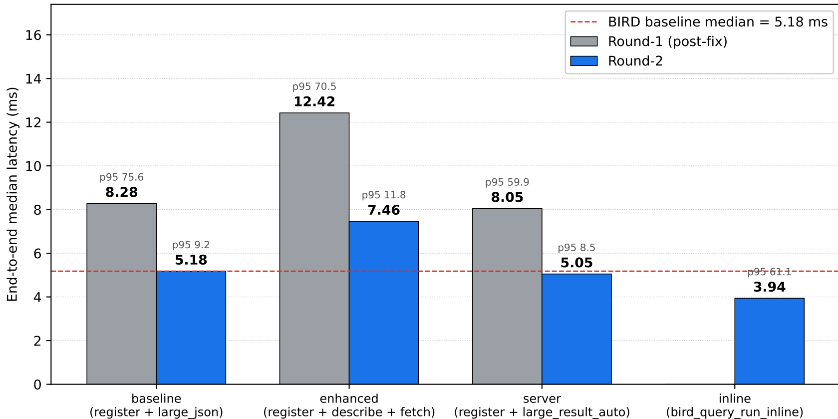
BIRD dev gold — end-to-end median latency per arm (p95 shown as label) Round-1 (post-fix) vs Round-2, n = 1534 queries
