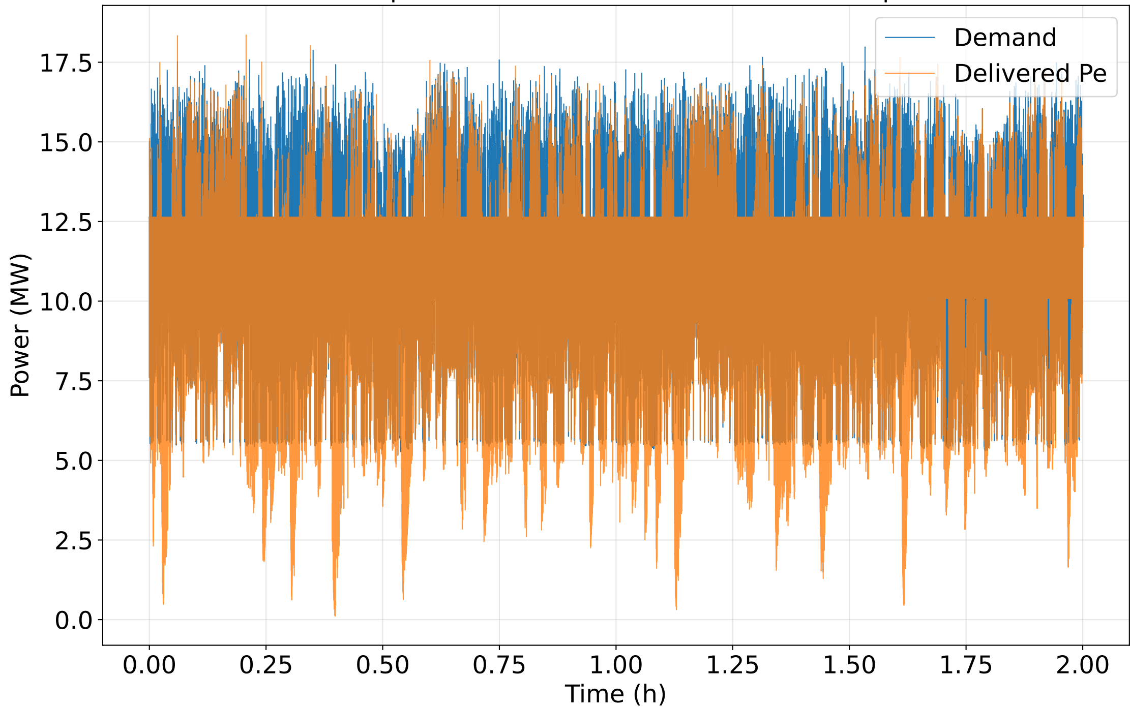
Tier C response: electrical demand and delivered power
