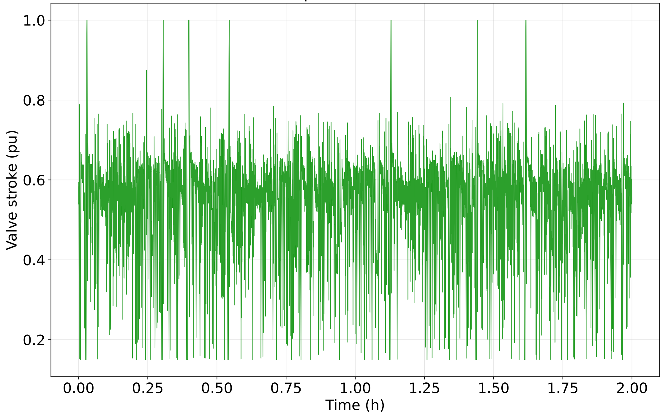
Tier C response: fuel valve stroke
