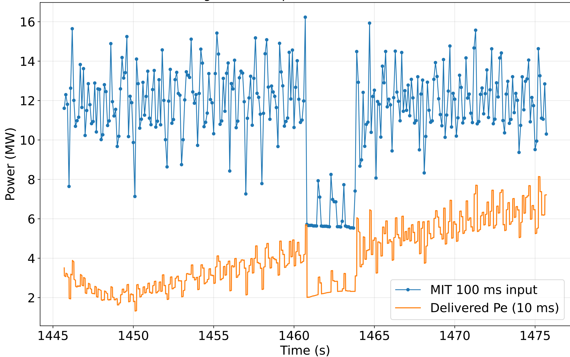
Zoom: governor response to 100 ms transients
