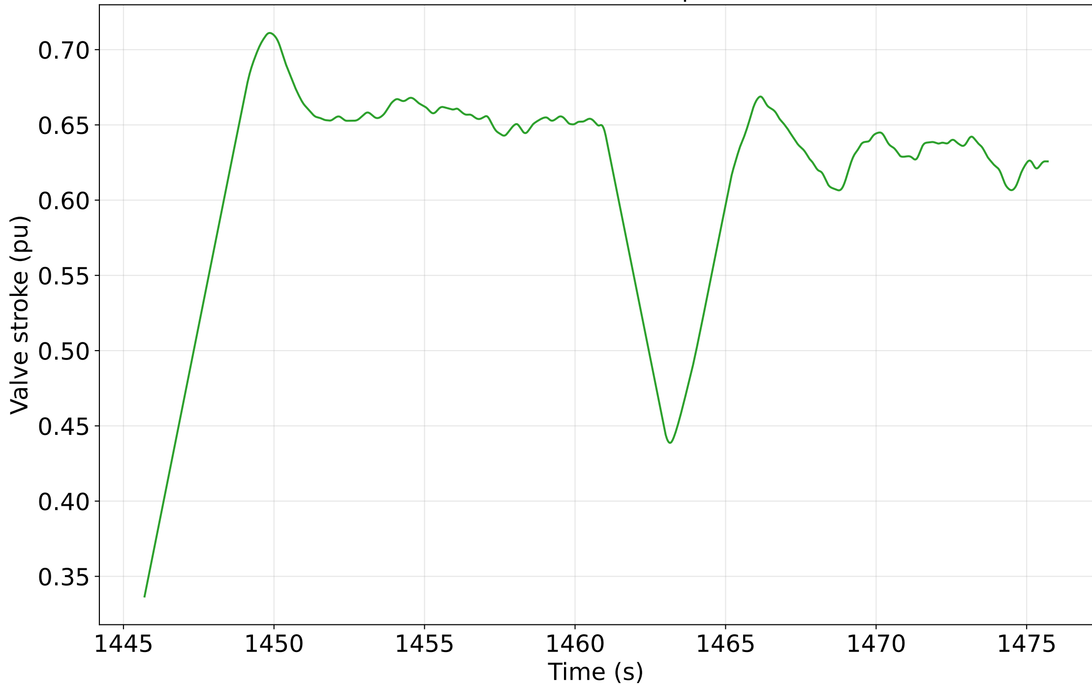
Zoom: fuel valve response
