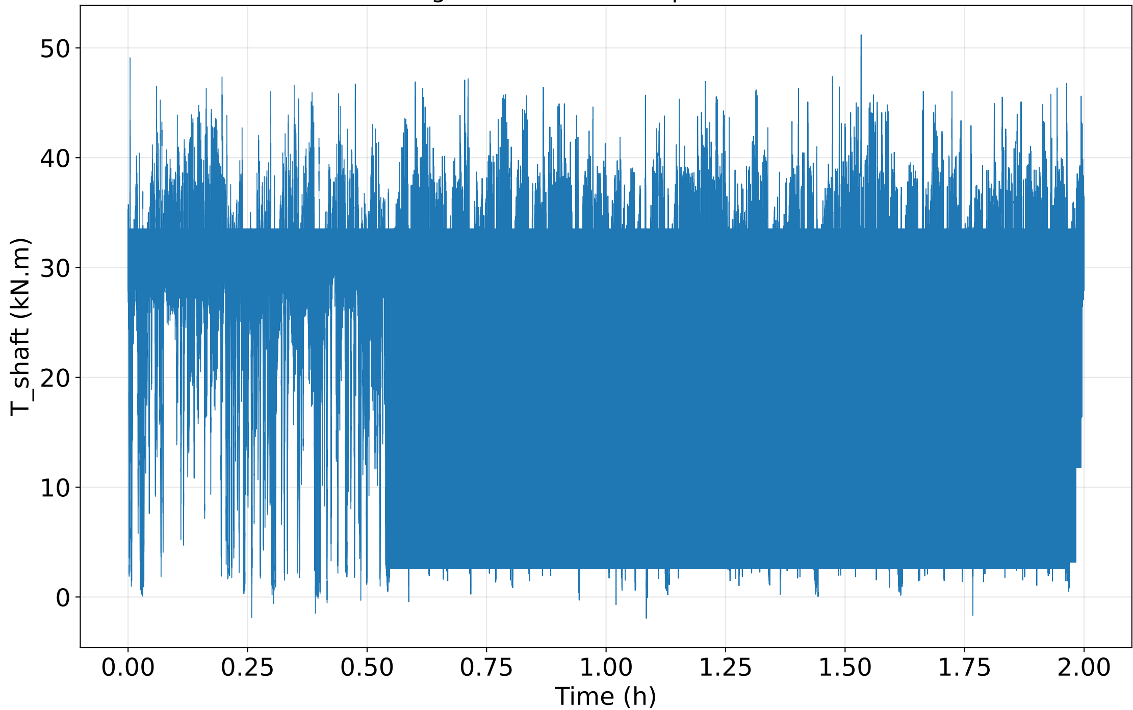
PT-generator shaft torque over 2 h
