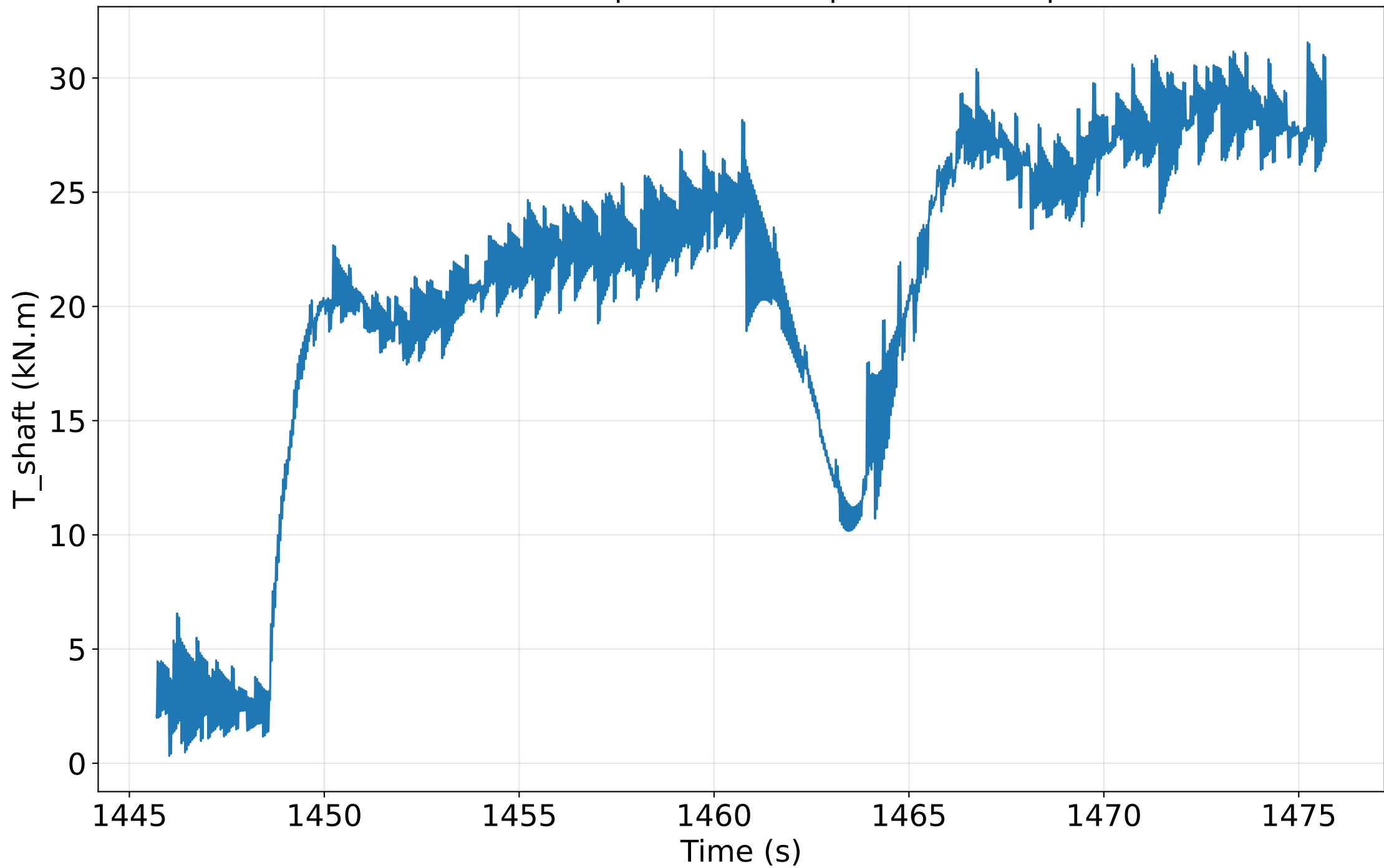
Zoom: torsional response around peak load-ramp event
