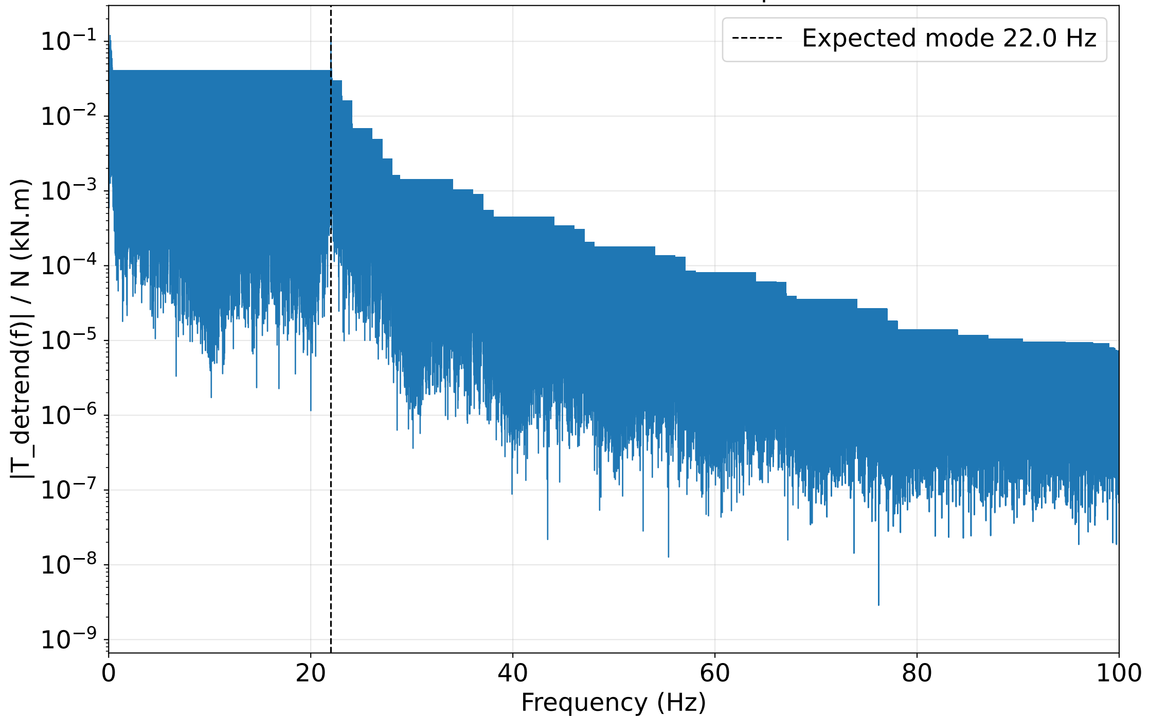
FFT of detrended shaft torque
