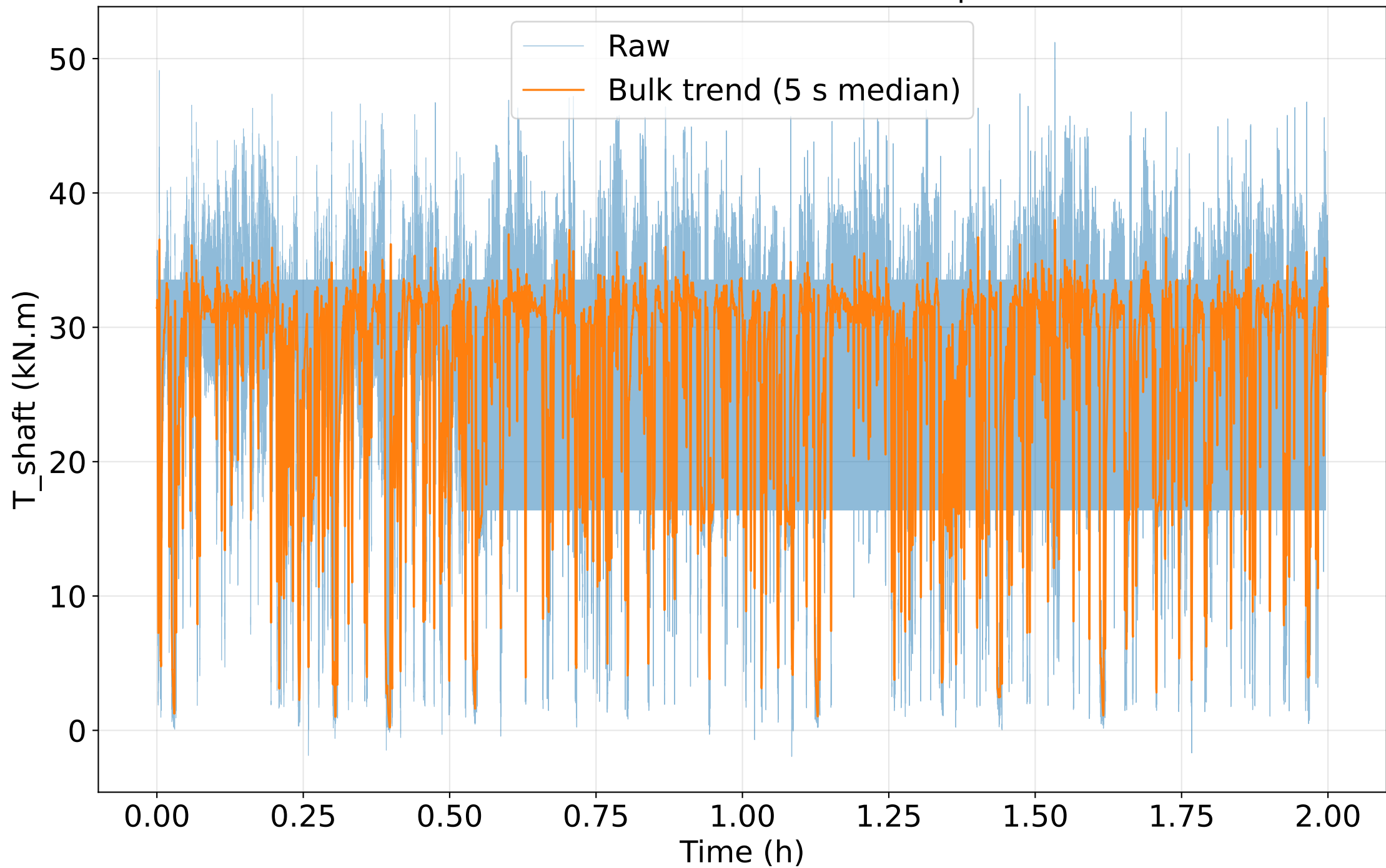
Bulk trend versus raw shaft torque
