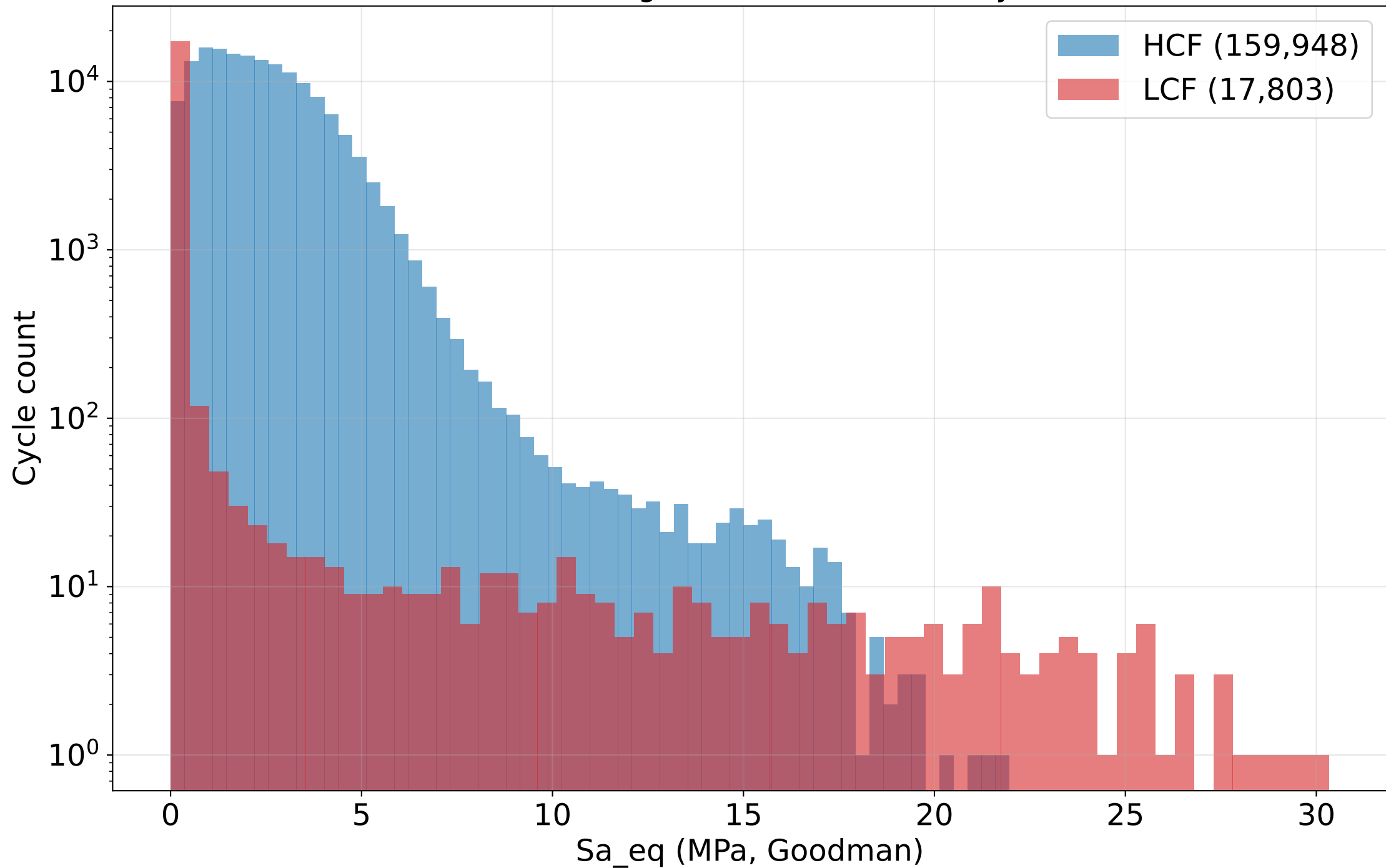
Rainflow histogram: HCF versus LCF cycles
