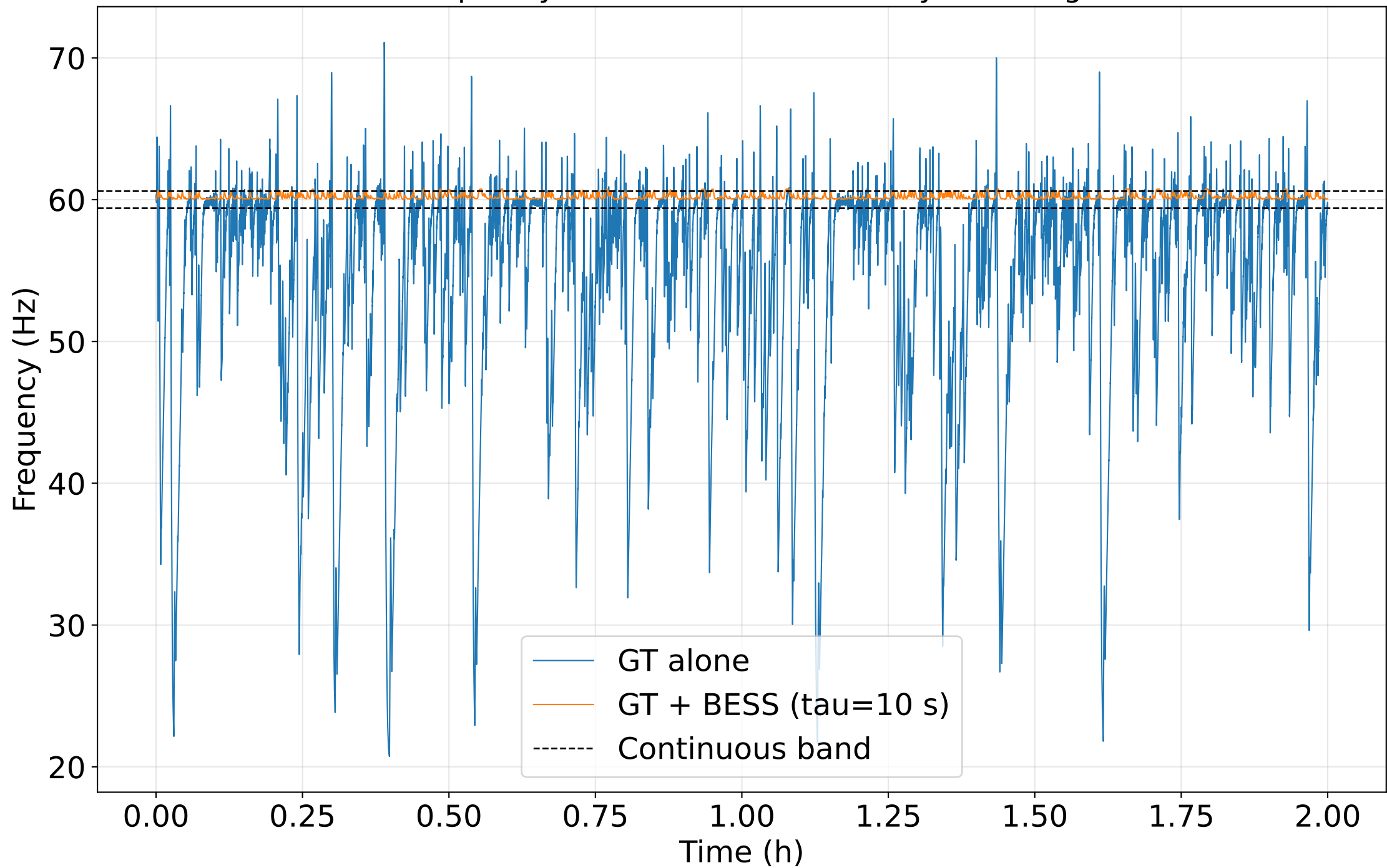
Frequency with and without battery buffering
