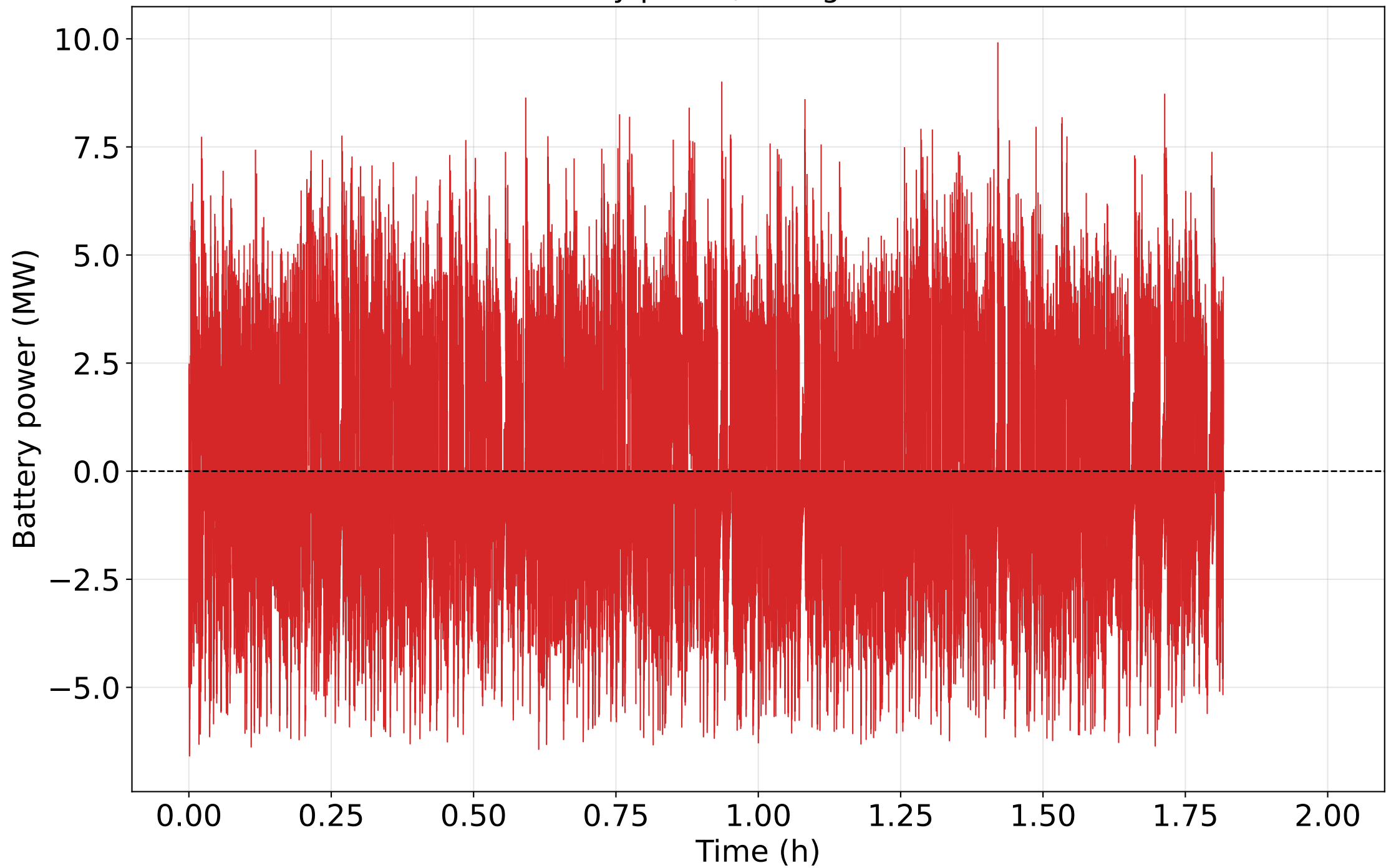
Battery power, rating = 9.9 MW
