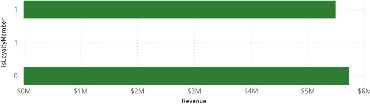
Segment Matrix
